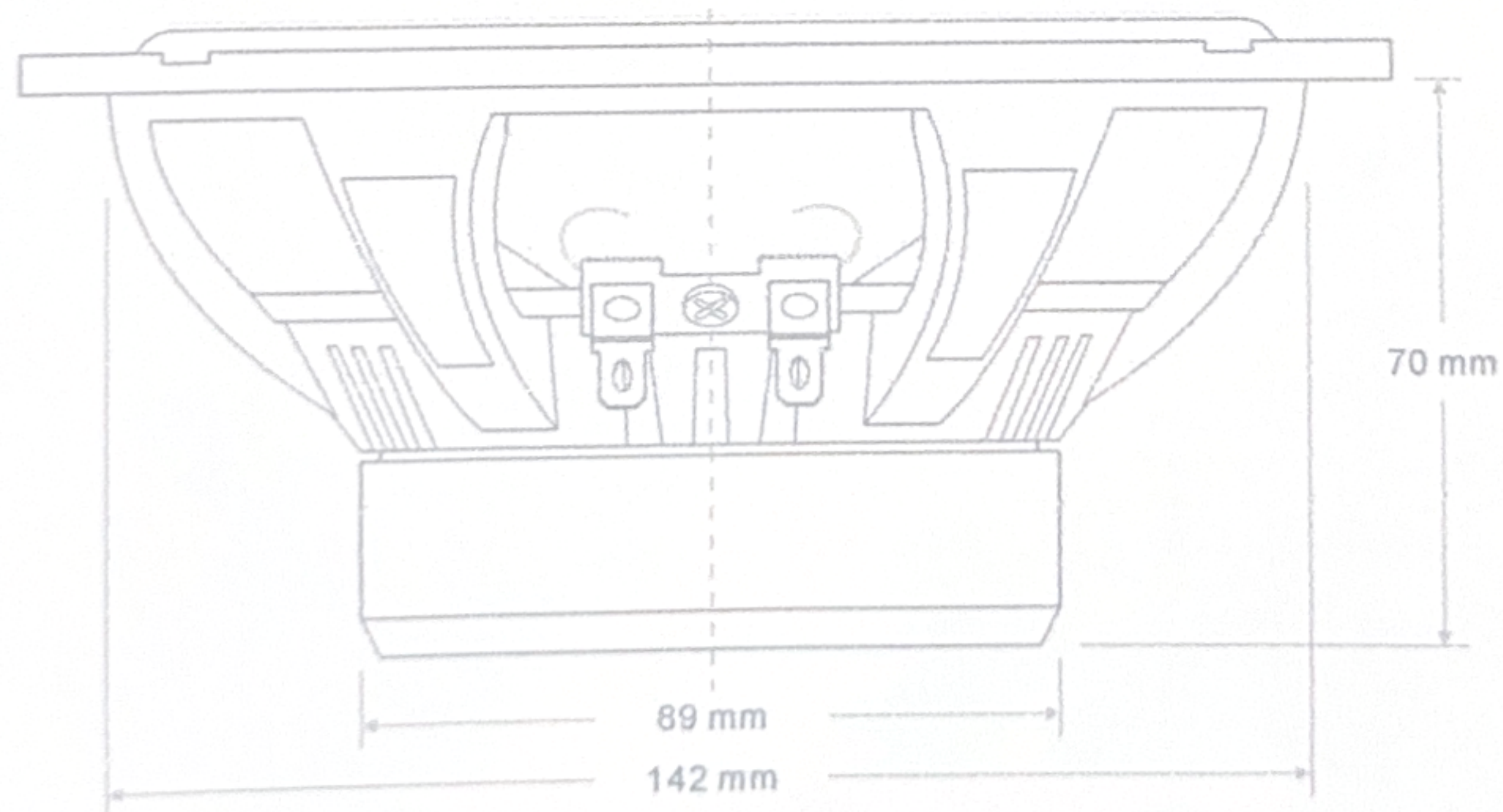
RL165 WOOFER
